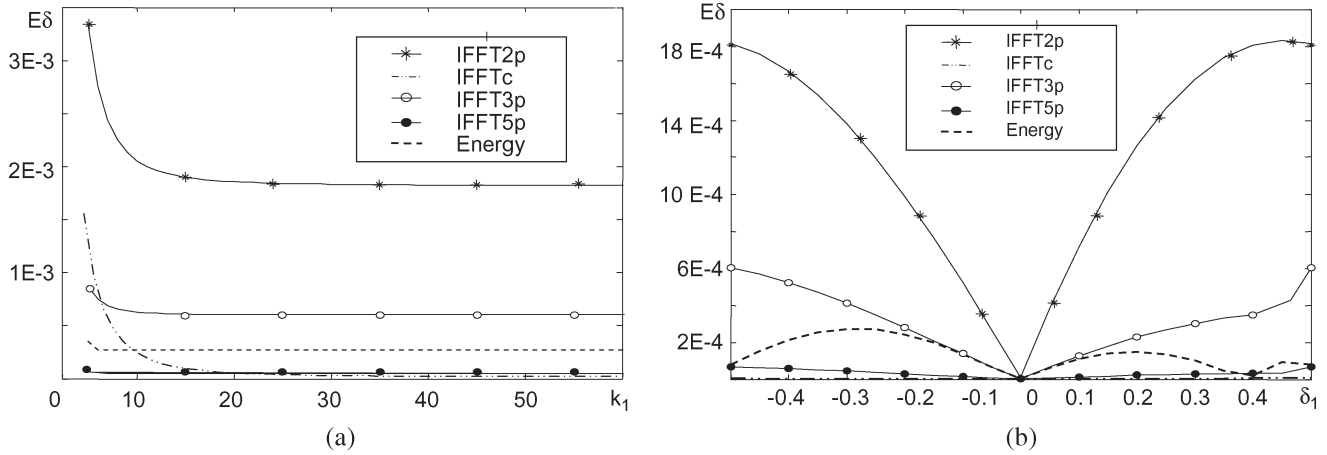
Fig. 1. For a signal with P = 2 , d_{12} = 10 , \beta_1 = \beta_2 = 1 ; f_1 = f_2 = 0 . (a) Maximum measured E_\delta for all possible values of \delta_1 versus k_1 . (b) E_\delta versus \delta_1 with k_1 = N/4 .
